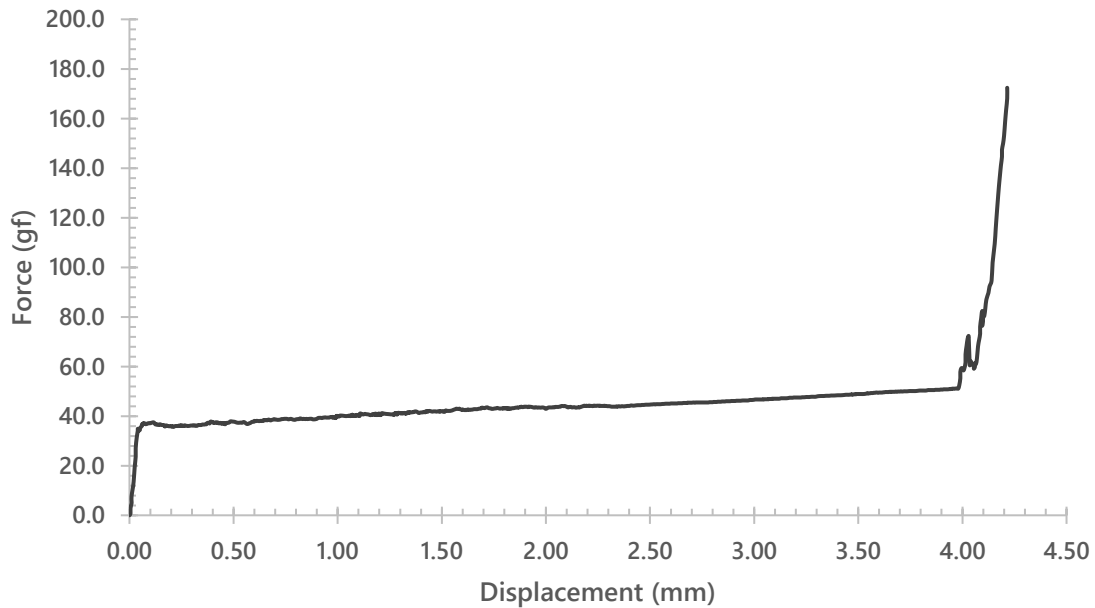
Douyu KBC-04-RD-TOR-4555-D (Upstroke)
